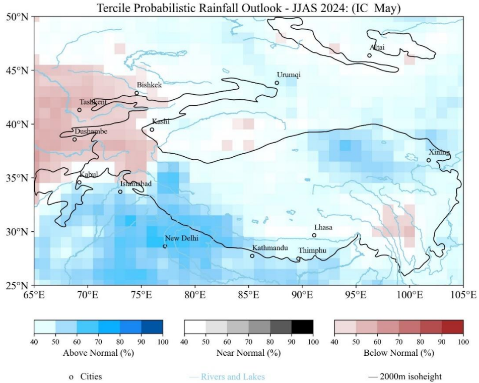
Figure 10 Precipitation Probabilistic outlook, JJAS 2024 for TP region
